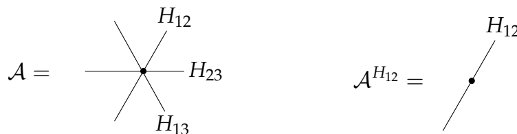
Figure 1: The rank-two braid arrangement (left) and its restriction at H_{12} (right).
